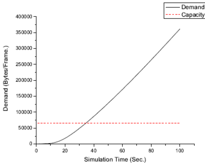
Fig.5.9. Total Bandwidth Demand
