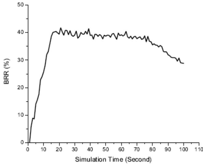
Fig 5.7. Simulation results of Bandwidth Recycling Rate (BRR).
