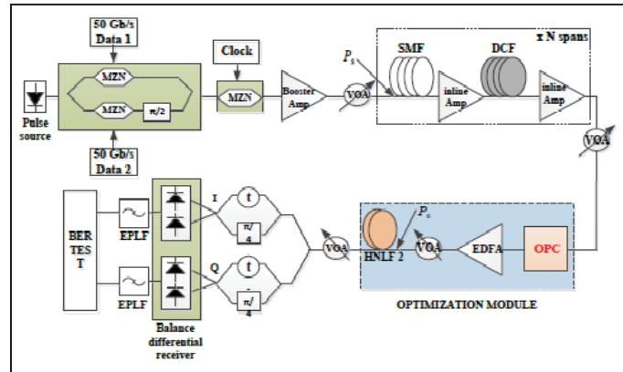
Fig. 1: Diagram of the System to be Analyzed.
