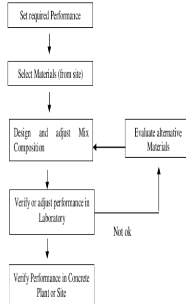
Figure1: SCC Mix Design Procedure (EFNARC, 2005) [3].
