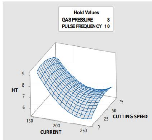
Figure 5. Graph of the Surface Cutting Velocity vs. HT vs. Current.
